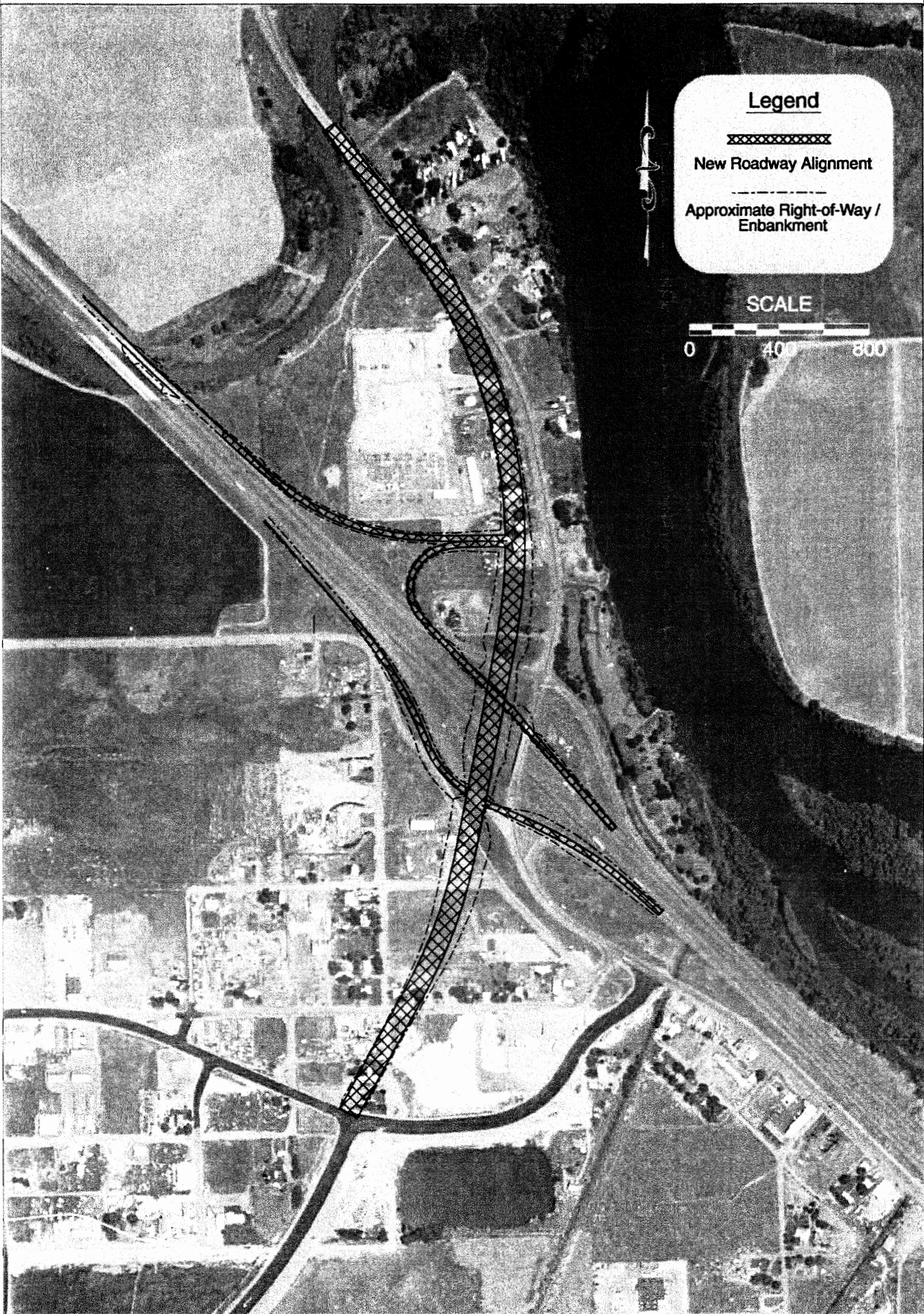
Alternative #8 Preferred Alignment & Interchange Form
