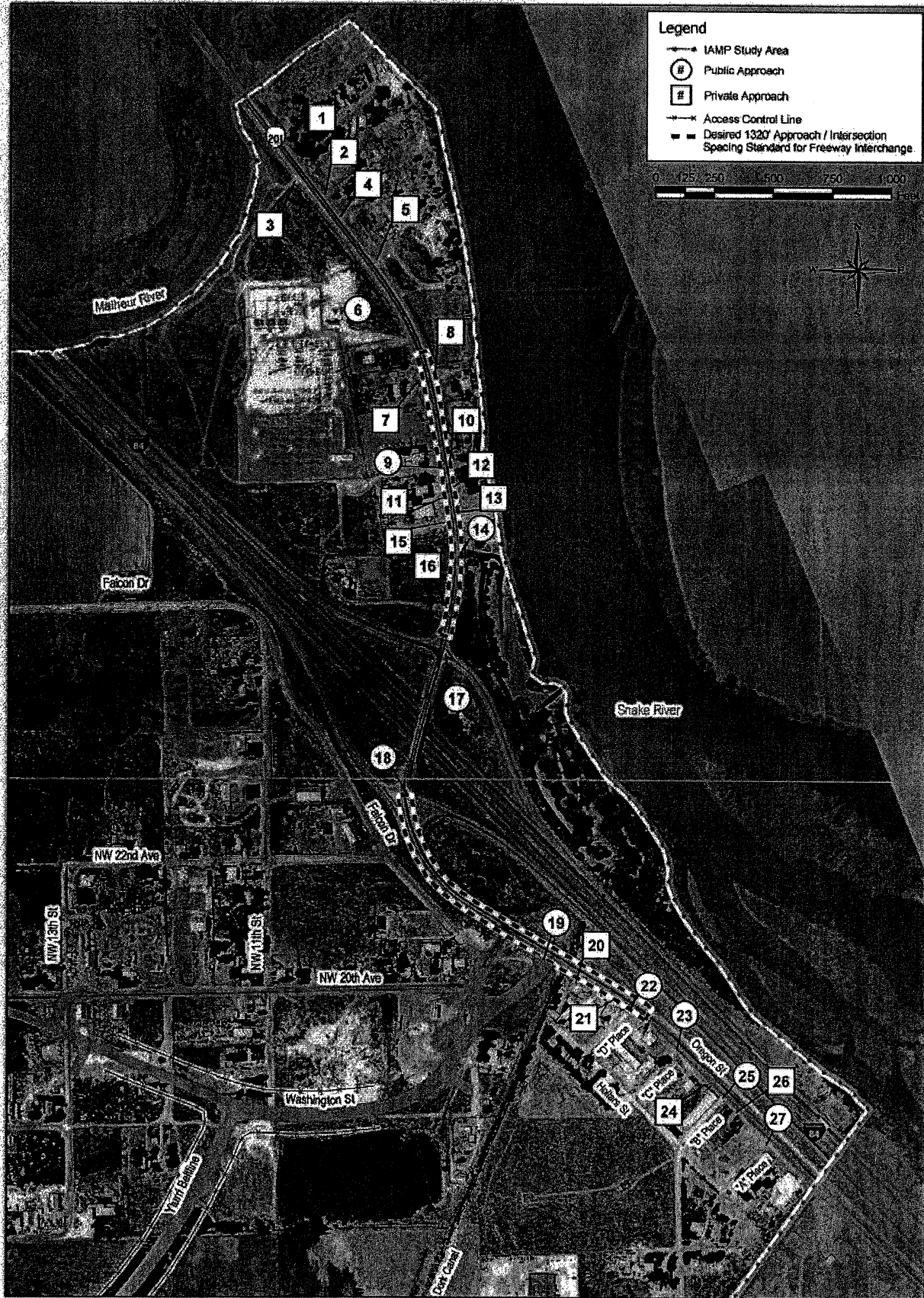
Existing OR201 Public/Private Access Locations
