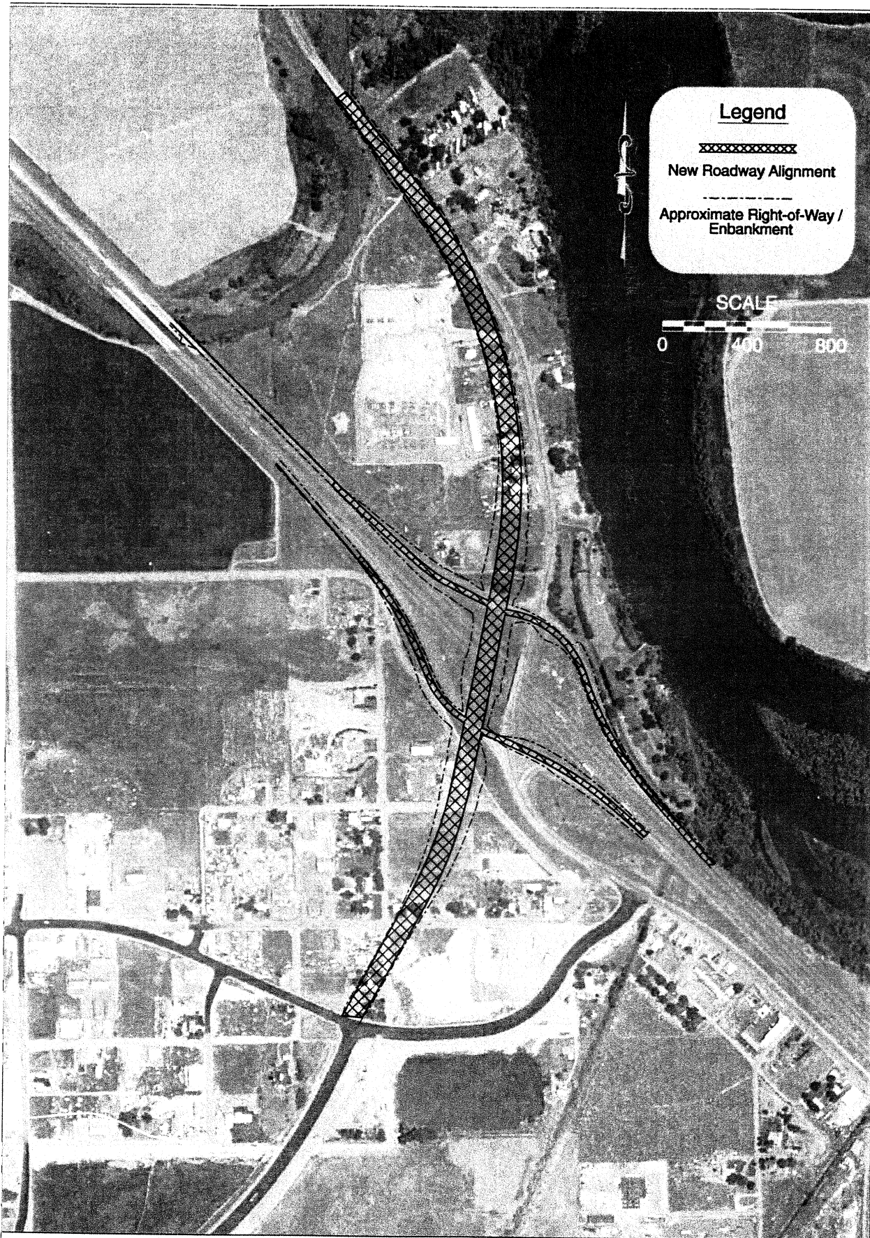
Alternative #10 Preferred Alignment & Interchange Form
