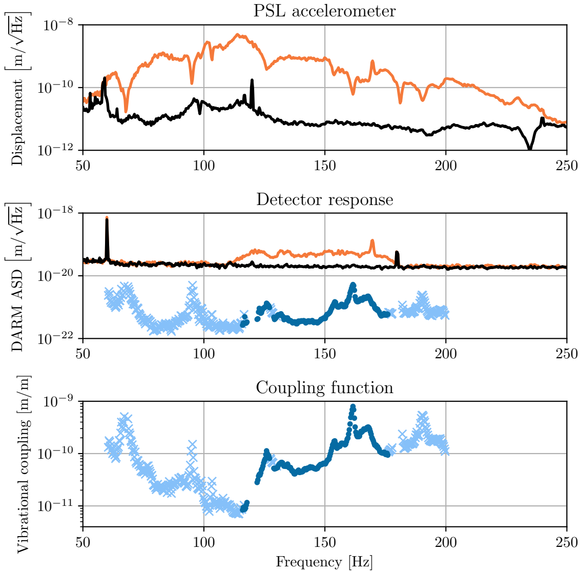
Figure 12. Example of a broadband acoustic noise injection and measurement of a single-injection coupling function. Top: displacement of an accelerometer in the PSL room during background time (black) and injection time (orange). Middle: DARM during background time (black) and injection time (orange). Estimated ambient levels for the accelerometer are shown as dark blue dots, with upper limits shown as light blue crosses. Bottom: single-injection coupling function used to produce estimated ambient above.
