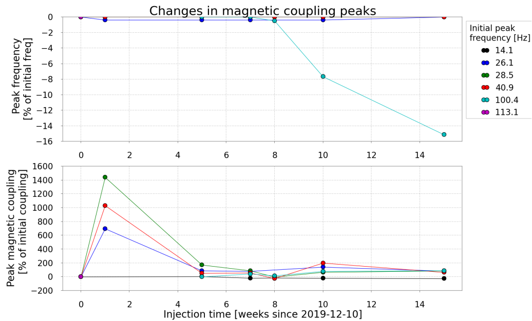
Figure 27. Weekly trends in frequency (top) and amplitude (bottom) of peaks in the magnetic coupling functions.
