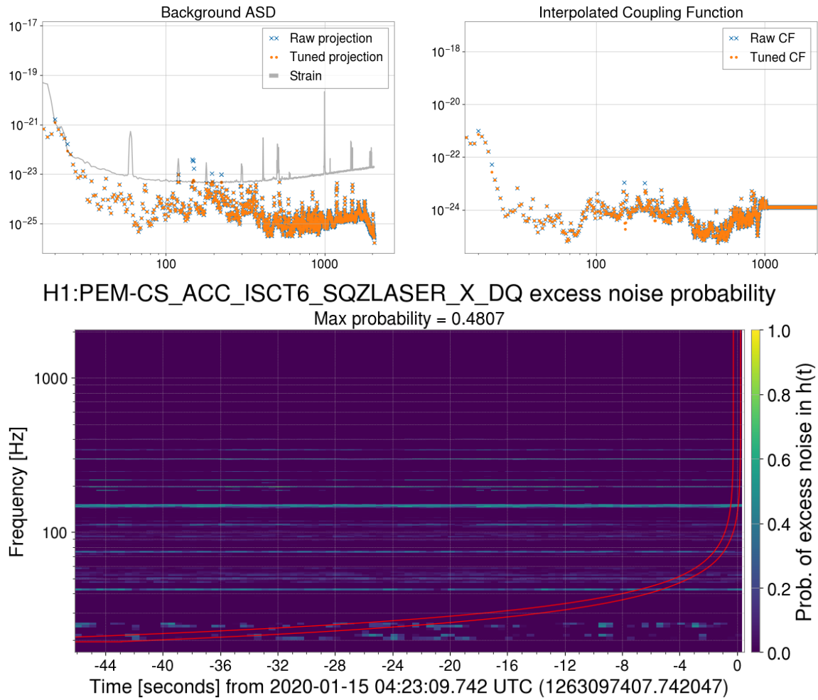
Figure 29. Coupling function tuning (top) and the resulting probability spectrogram (bottom).
