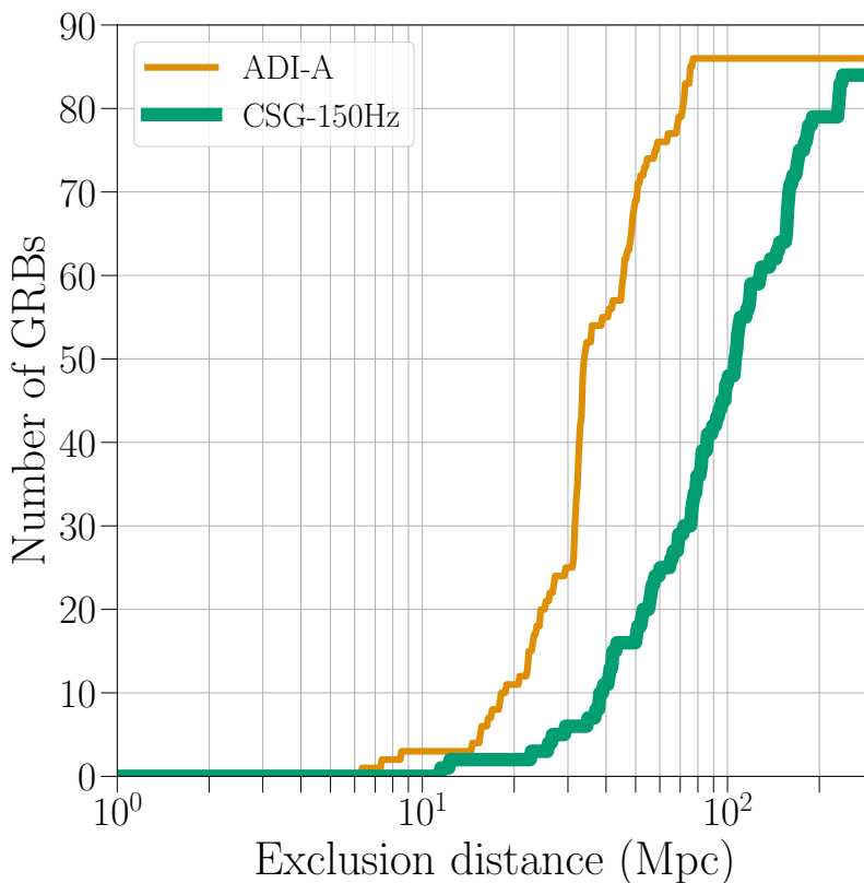
Figure 36. Cumulative distributions of O3b exclusion distances for 150-Hz sine-Gaussian and ADI-A waveforms.
