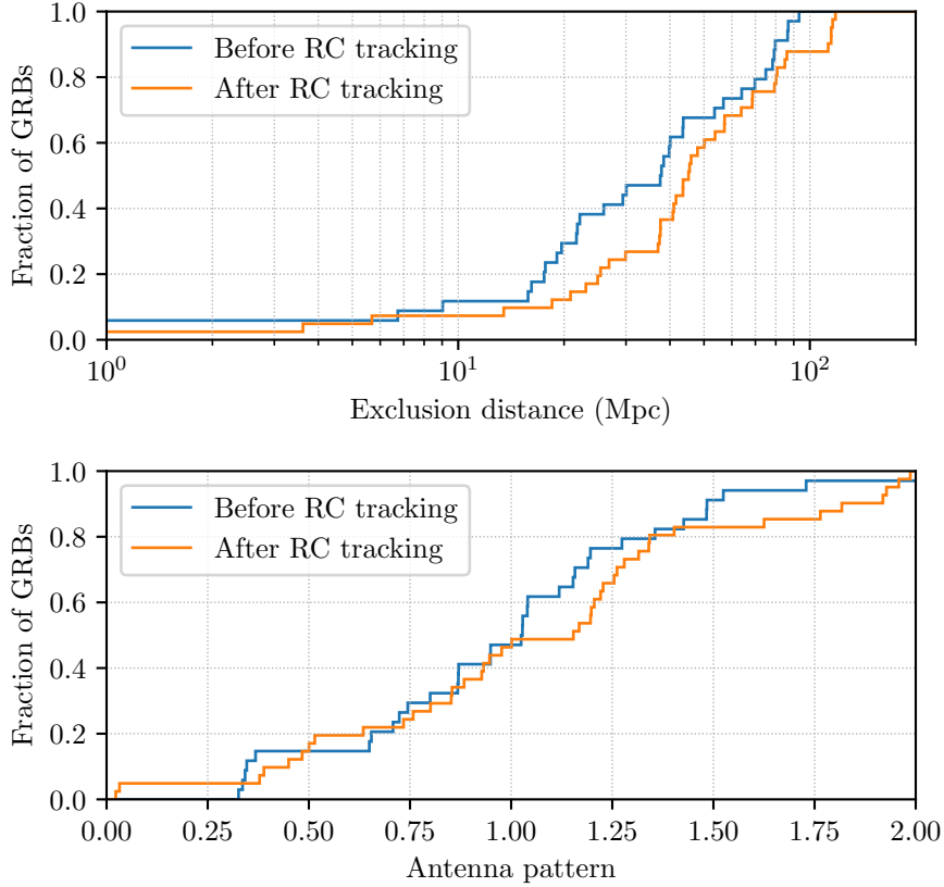
Figure 38. Cumulative distributions of CSG-300 Hz exclusion distances (top) and the detector network antenna factors (bottom) for GRBs before and after the implementation of RC tracking.
