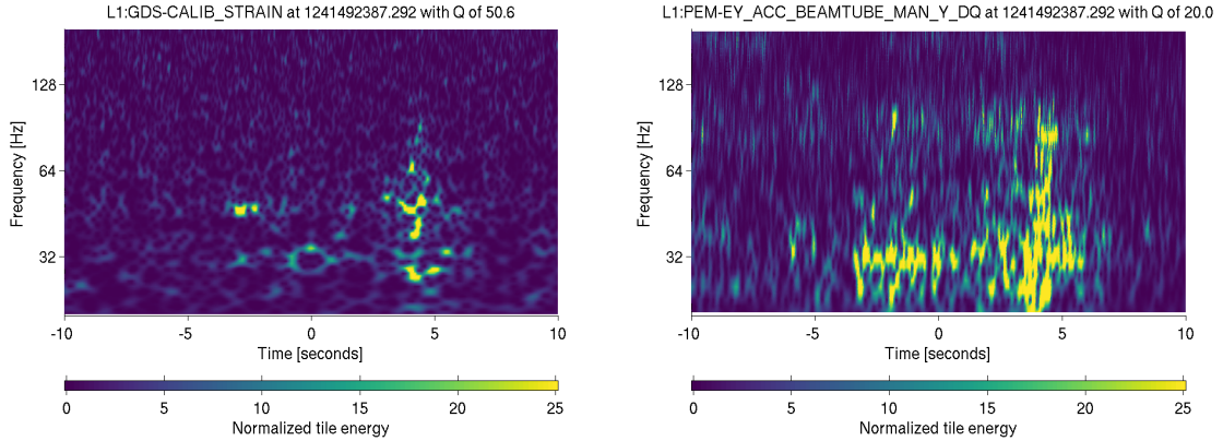
Figure 16. Constant-Q transforms of the GW strain channel (left) and an accelerometer (right) during thunder noise at LLO.
