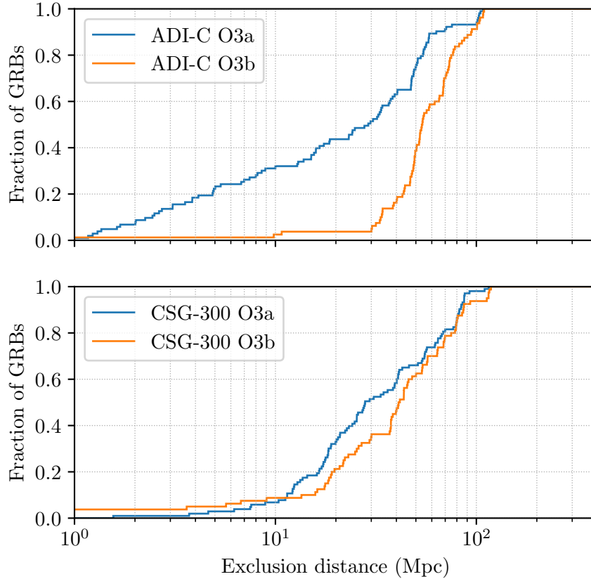
Figure 37. Cumulative distributions of O3a and O3b exclusion distances for the ADI-C (top) and 300-Hz sine-Gaussian (bottom) waveforms. These show the greatest improvement between O3a and O3b among their respective waveform sets.
