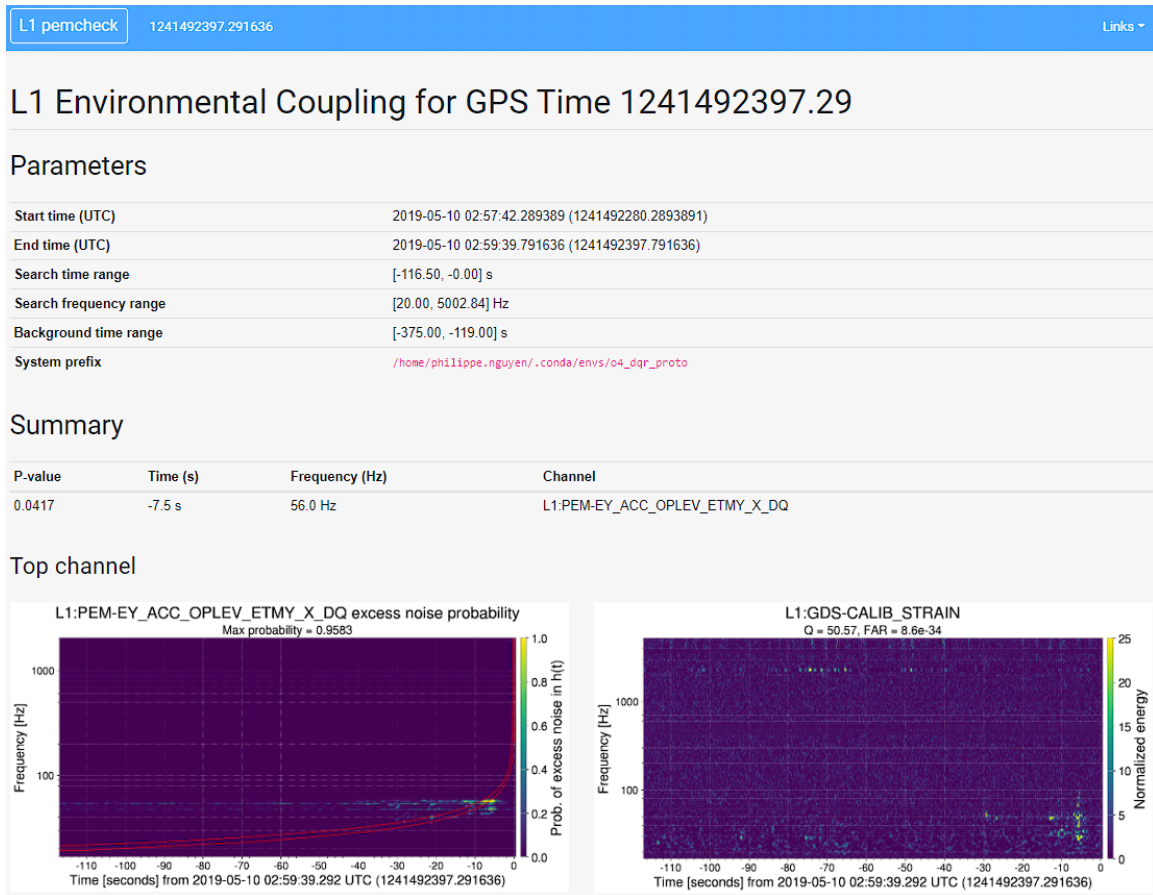
Figure B.1. Example for a long duration CBC merger candidate S190510g, overlapping with excess noise that is almost certainly associated with vibrational noise at ETMY.
