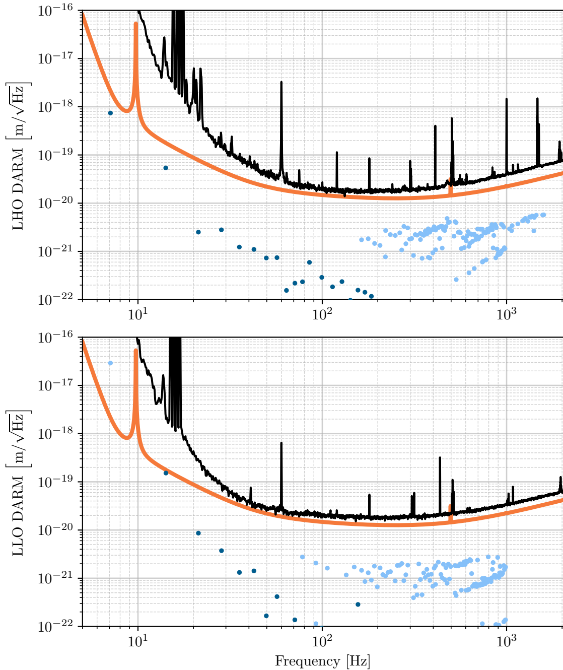
Figure 24. DARM noise from all magnetic coupling sources at LHO (top) and LLO (bottom). Dark blue dots represent measurements, while light blue dots represent upper limits. The black and orange curves show the O3 sensitivity and design sensitivity, respectively.
