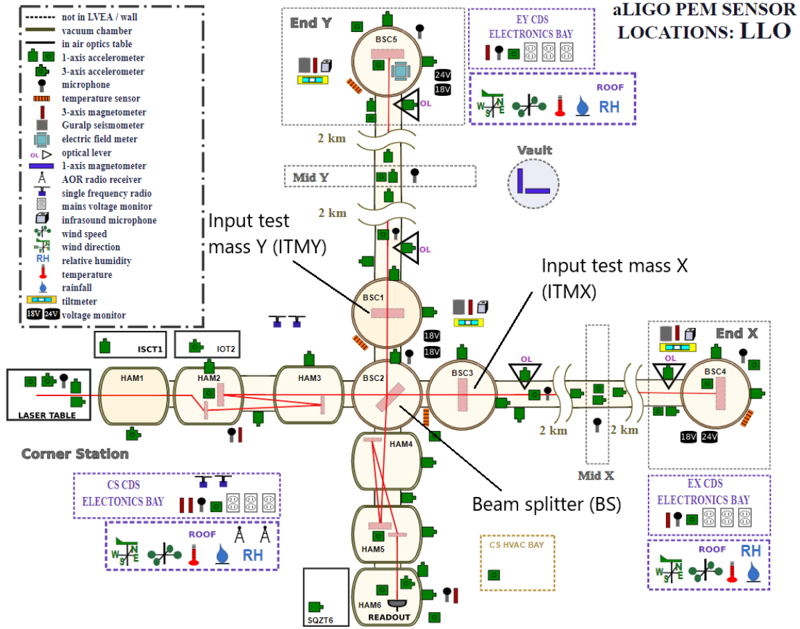
Figure 6. The PEM system layout at LLO during O3, as seen on the PEM public website ( pem.ligo.org ).
