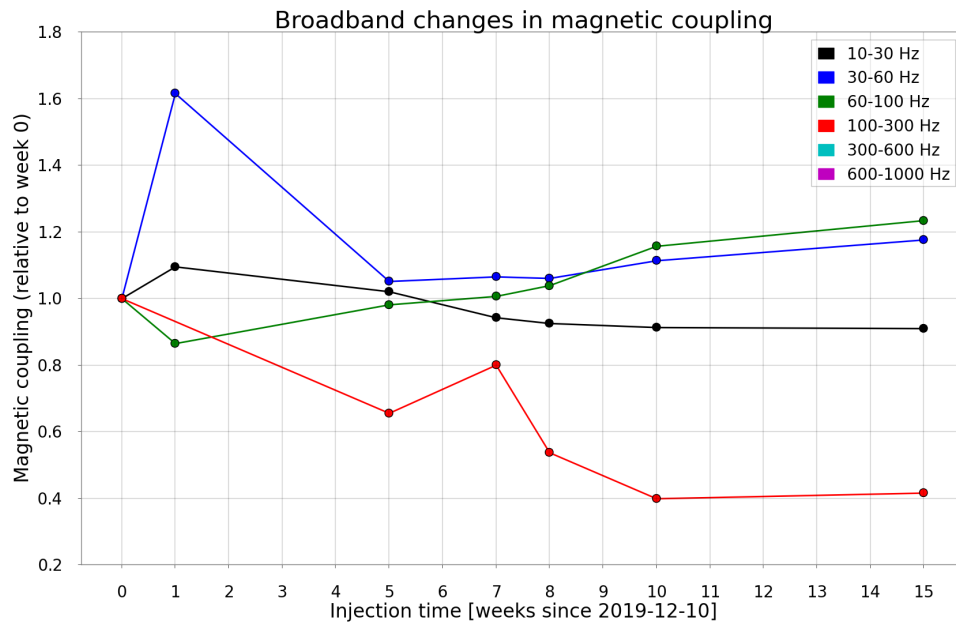
Figure 26. Time-lines of magnetic coupling changes relative to the start of the observing run.
