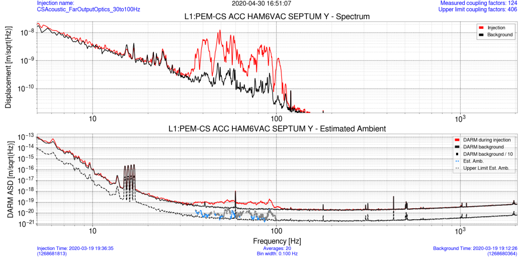
Figure A.4. Estimated ambient for the Y-axis HAM 5/6 septum accelerometer from a broadband acoustic injection.
