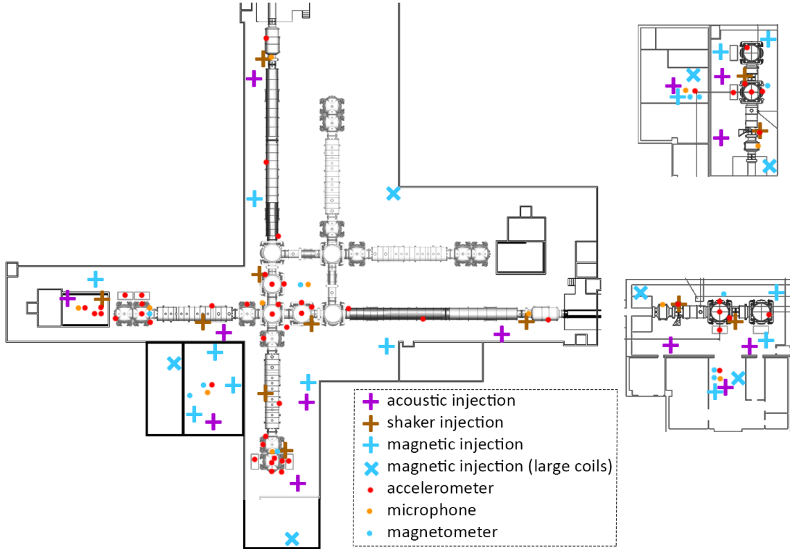
Figure 8. Standard locations for vibration and magnetic injections at the LHO corner station (left), Y end station (top right), and X end stations (bottom right).
