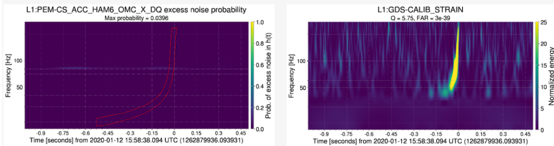
Figure B.3. Example of a typical short-duration CBC merger candidate S200112r, with no excess noise expected to appear in the GW channel.
