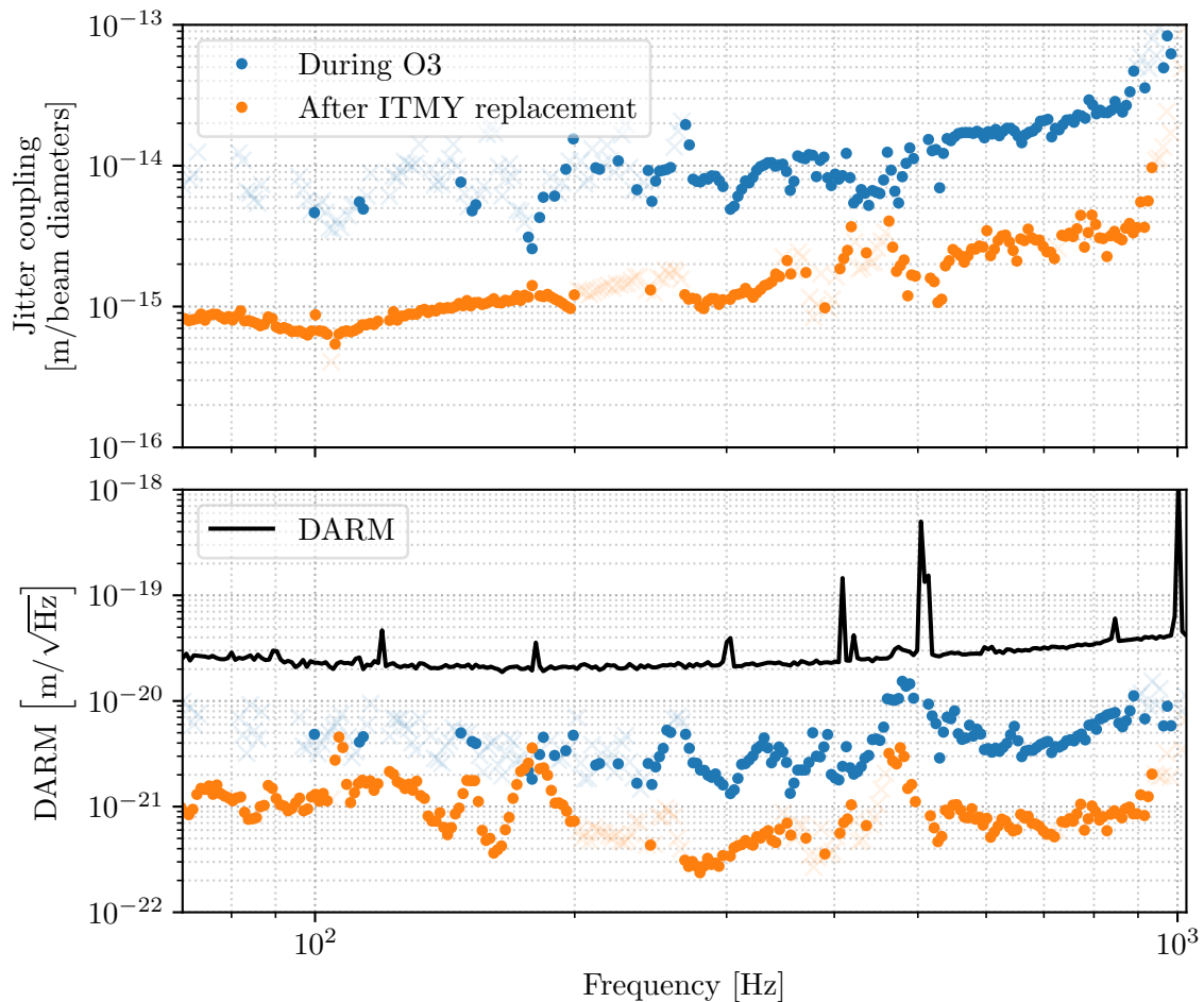
Figure 23. Improvement in jitter coupling at LHO after test mass replacement.
