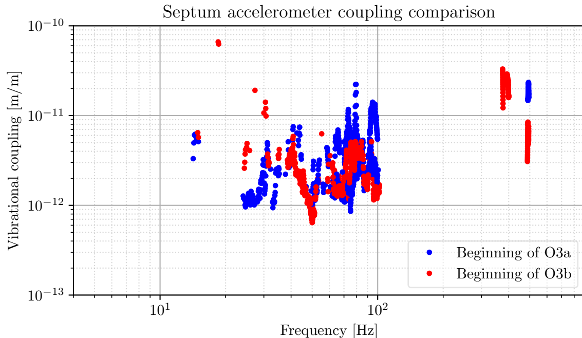
Figure 20. Change in HAM5/6 vibrational coupling before and after the replacement of the septum window.
