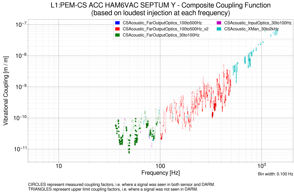
Figure A.5. Composite coupling function in physical units for the Y-axis HAM 5/6 septum accelerometer.
