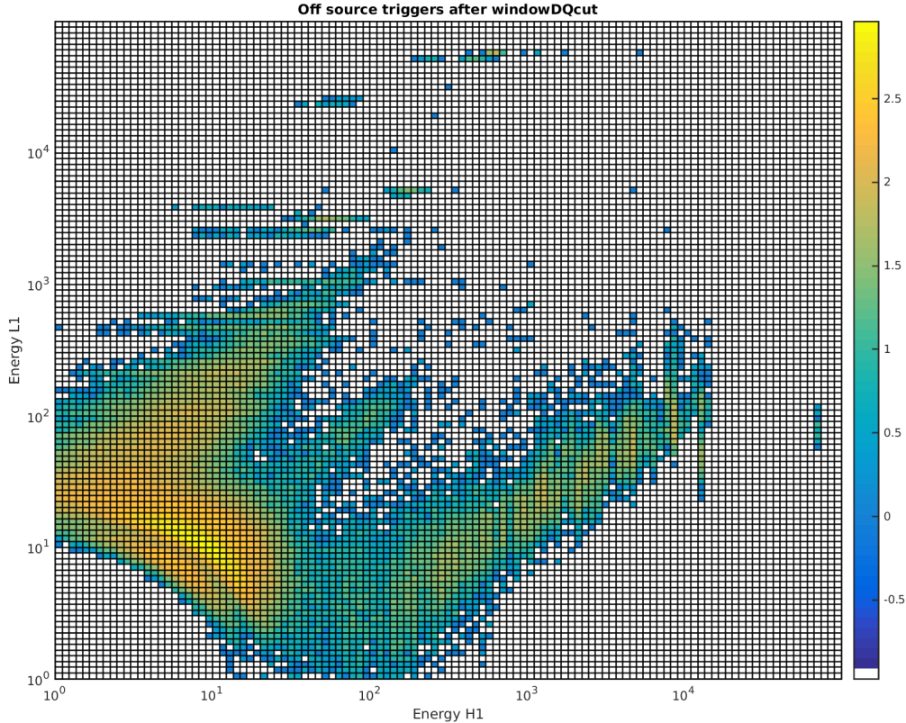
Figure 33. Distribution of off-source triggers in the LIGO detectors without autogating. The x- and y-axes are the signal energy in H1 and L1, respectively.
