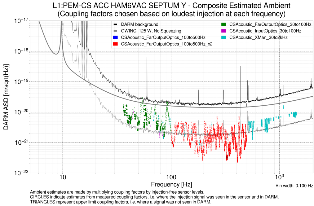
Figure A.7. Estimated ambient for the Y-axis HAM 5/6 septum accelerometer.
