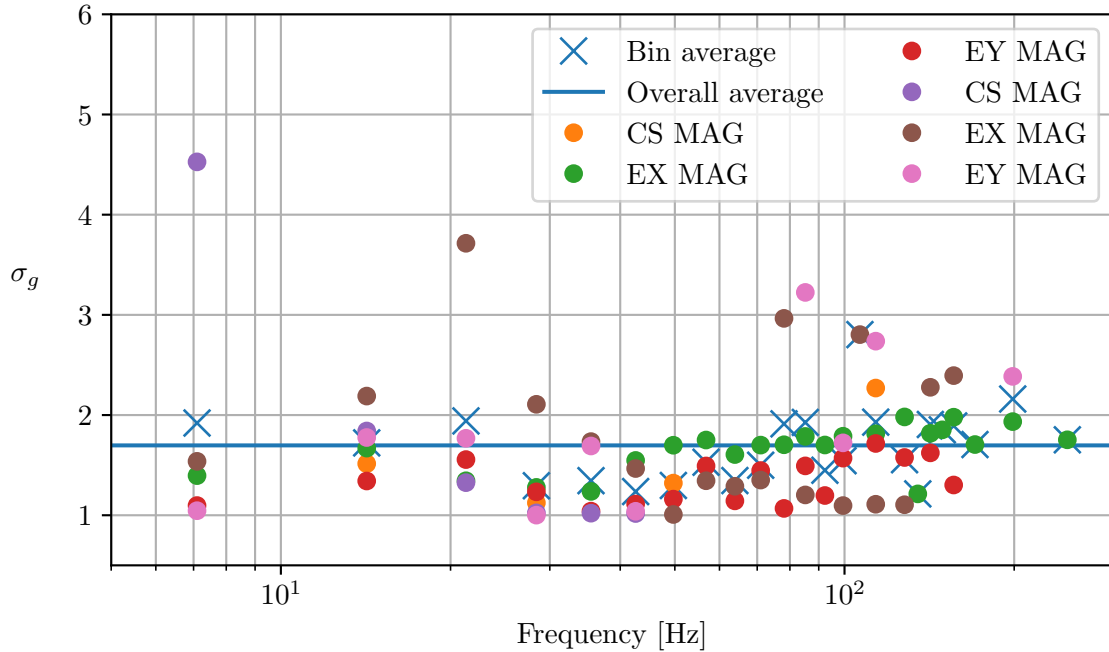
Figure 15. Magnetic coupling function uncertainty. Points show geometric standard deviations of magnetic coupling measurements when varying the injection location.
