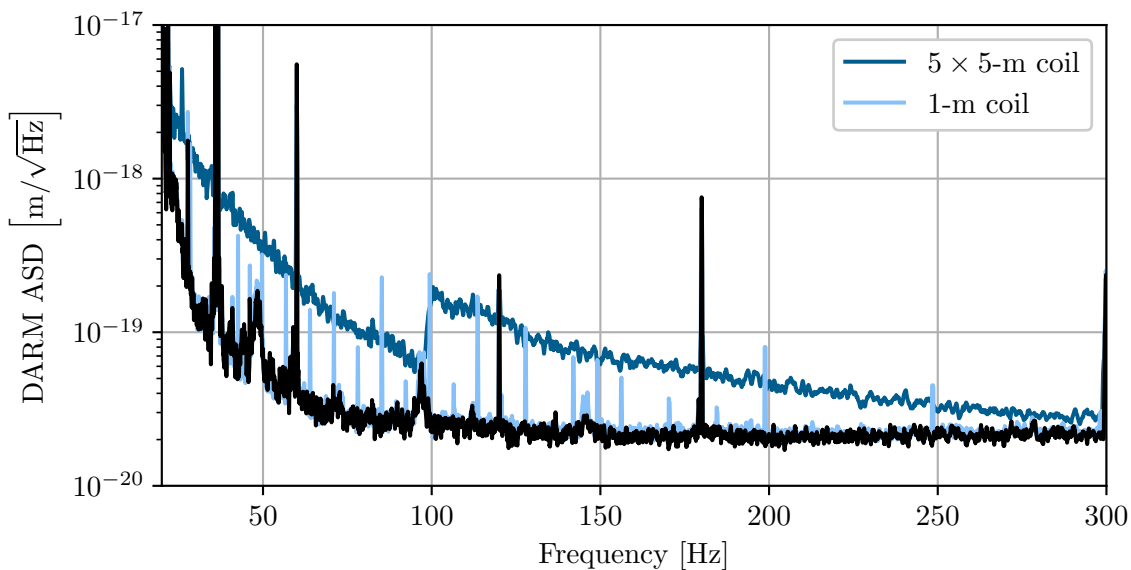
Figure 9. Comparison of the old small-coil comb magnetic field injections with the new large-coil broadband injections.
