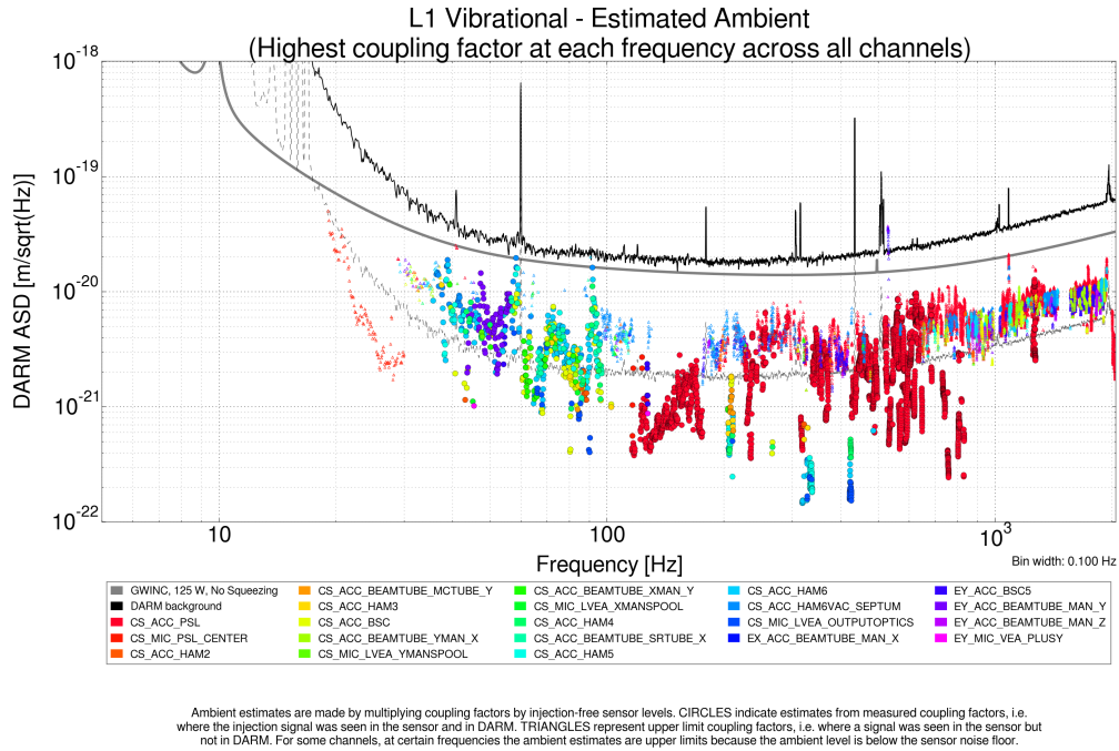
Figure A.8. Site-wide estimated ambient for all vibrational sensors at LLO.
