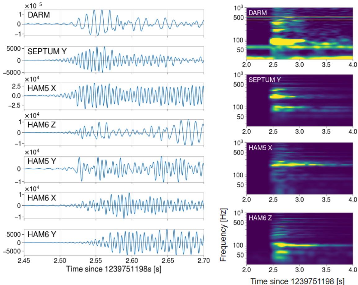
Figure 19. Time series (left) and spectrograms (right) of DARM and various accelerometers observing a vibrational impulse injection produced at the output arm of the LHO detector.
