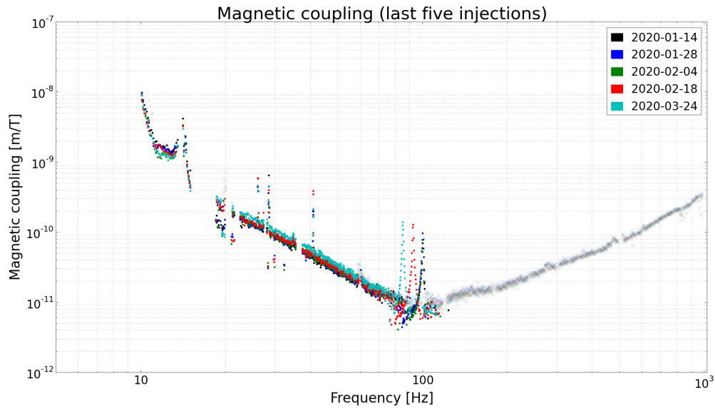
Figure 25. LHO magnetic coupling measured by the last five wall-mounted coil injections performed in O3.
