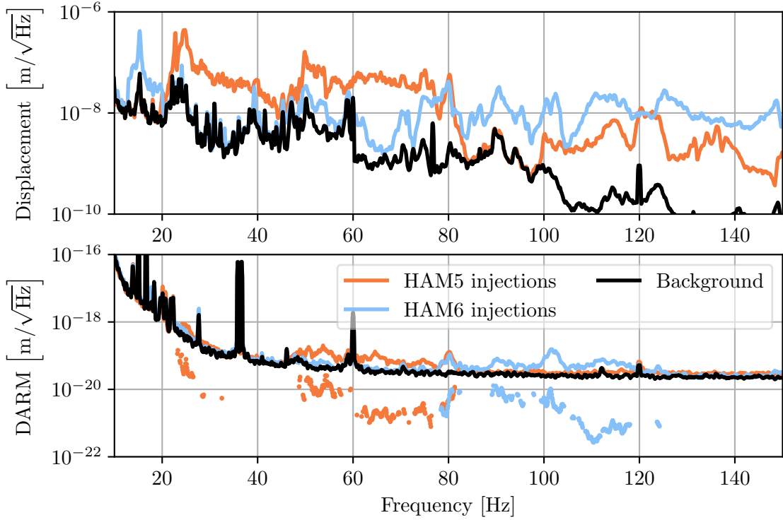
Figure 18. Spectra of shaker injections exciting scattered light noise at the LHO output arm. Top: Injections observed by the HAM5/6 septum accelerometer, stitched together from multiple bandpassed injections (each covering a 20-Hz range). Bottom: DARM responses to the injections (solid lines) and estimated ambients from coupling functions in dots.
