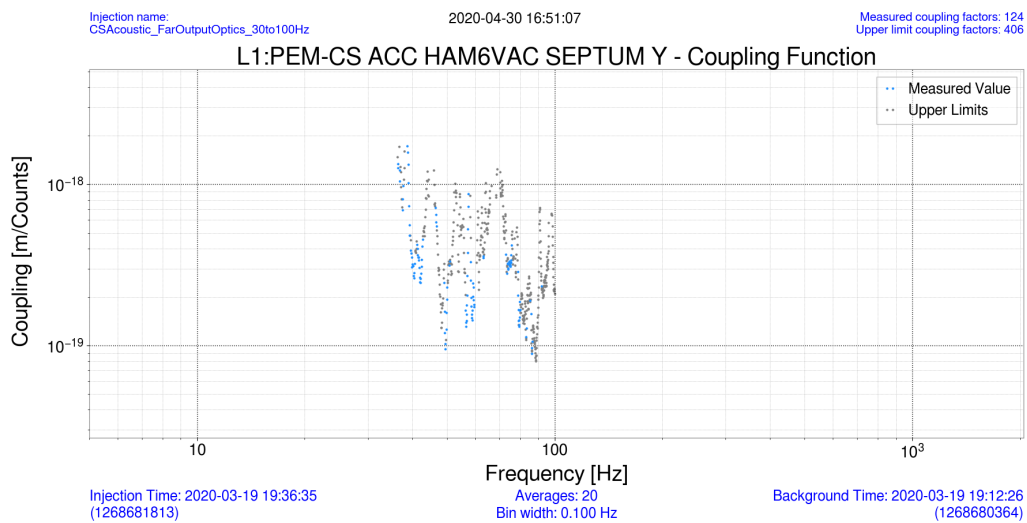
Figure A.3. Coupling function in ADC counts for the Y-axis HAM 5/6 septum accelerometer from a broadband acoustic injection.
