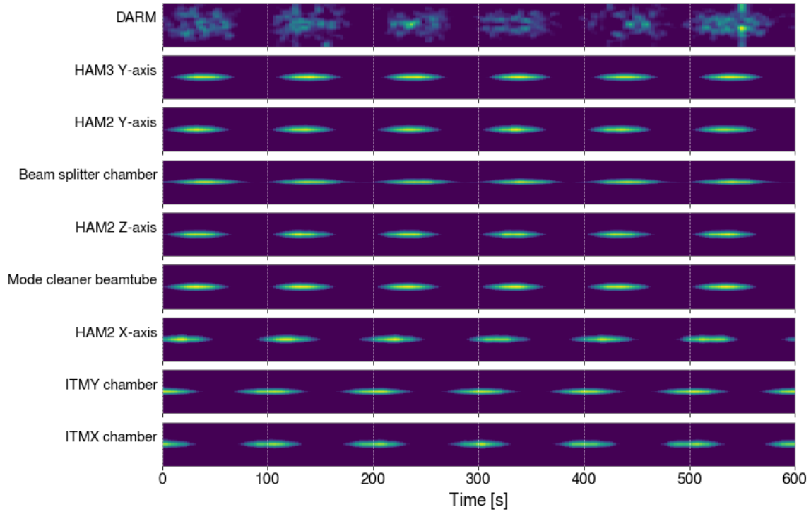
Figure 22. Spectrograms of DARM and various accelerometers near the input arm and beam splitter showing a beating-shakers injection at 48 Hz.
