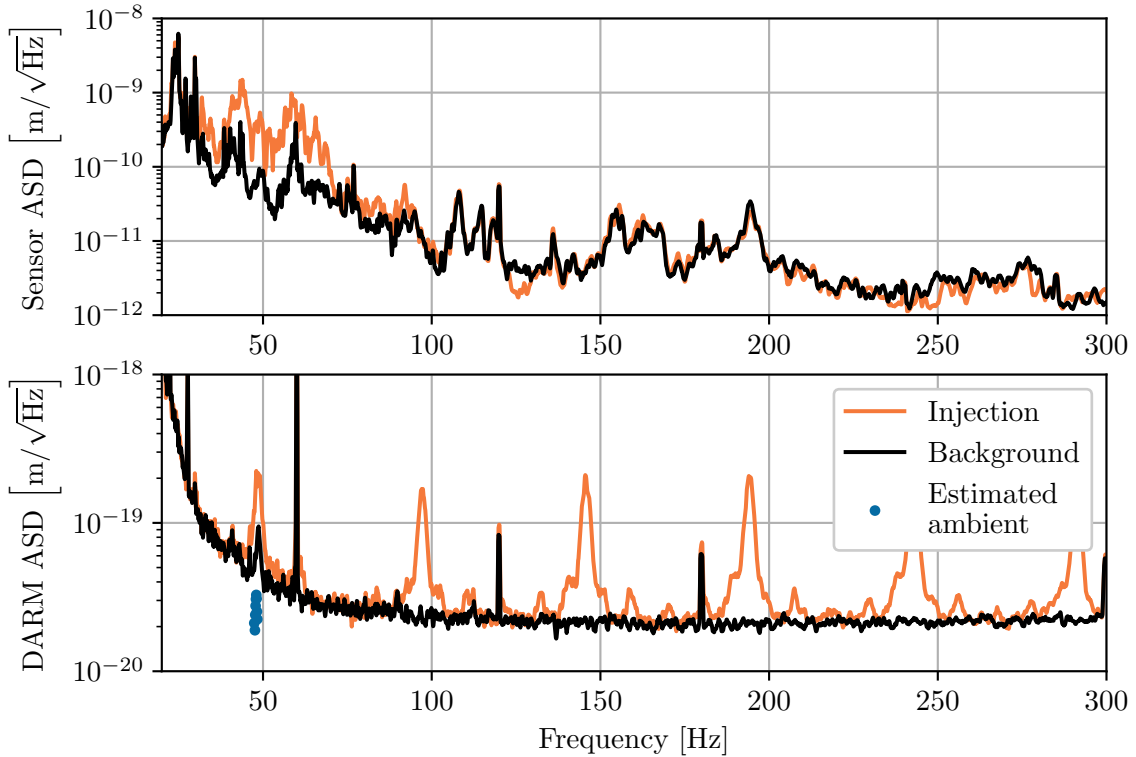
Figure 21. ASD of a vibrational injection measured by a HAM3 accelerometer (top) at the LHO input arm exciting a 48-Hz resonance feature in DARM (bottom).
