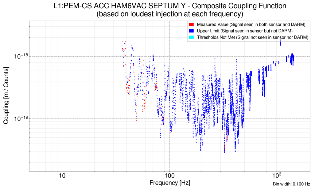
Figure A.5. Composite coupling function in physical units for the Y-axis HAM 5/6 septum accelerometer.
