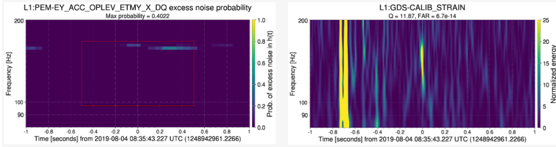
Figure B.2. Example for a burst candidate S190804qr reported by cWB, showing that a loud noise observed near ETMY could contribute to the GW event candidate signal but not with a high probability.
