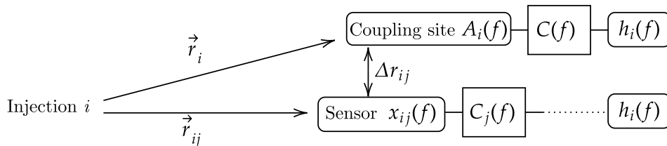
Figure 10. Diagram of a coupling function measurement in the trivial case. An injection i produces a signal A_i(f) at a coupling site, which cannot be measured directly. If the injection is performed sufficiently far from the sensor, then \Delta r_{ij} \ll \|\vec{r}_{ij}\| , so C_j(f) \approx C(f) .
