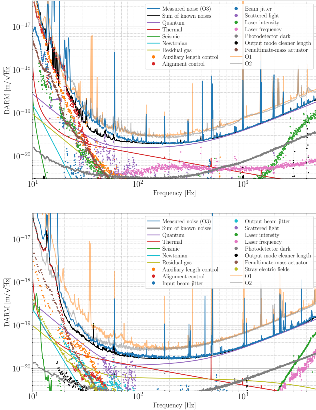
Figure 5. Full noise budgets of the LIGO Hanford (top) and Livingston (bottom) observatories at the end of the third observing run. Quantum noise refers to both shot noise and radiation pressure noise. Reproduced from Buikema et al. (2020).
