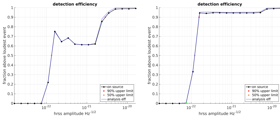
Figure 34. Detection efficiency of ADI-C injected waveforms without (left) and with (right) autogating.
