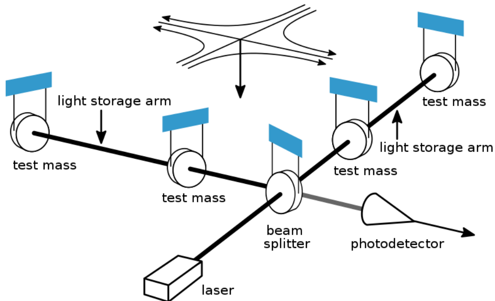
Figure 3. Layout of a Michelson interferometer with Fabry-Pérot arm cavities.
