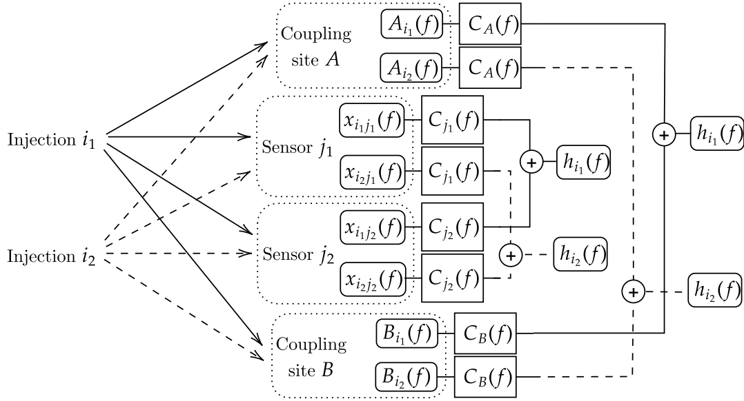
Figure 11. Expanding Figure 10 to two injections i_1 and i_2 , two sensors j_1 and j_2 , and two coupling sites A and B . Each injection response h_i(f) is itself a sum across contributions from A and B . The goal is to determine the sensor couplings C_j(f) that reproduce h_i(f) using the sensor measurements x_{ij}(f) since the true coupling actuations A_i(f) and B_i(f) are not known.
