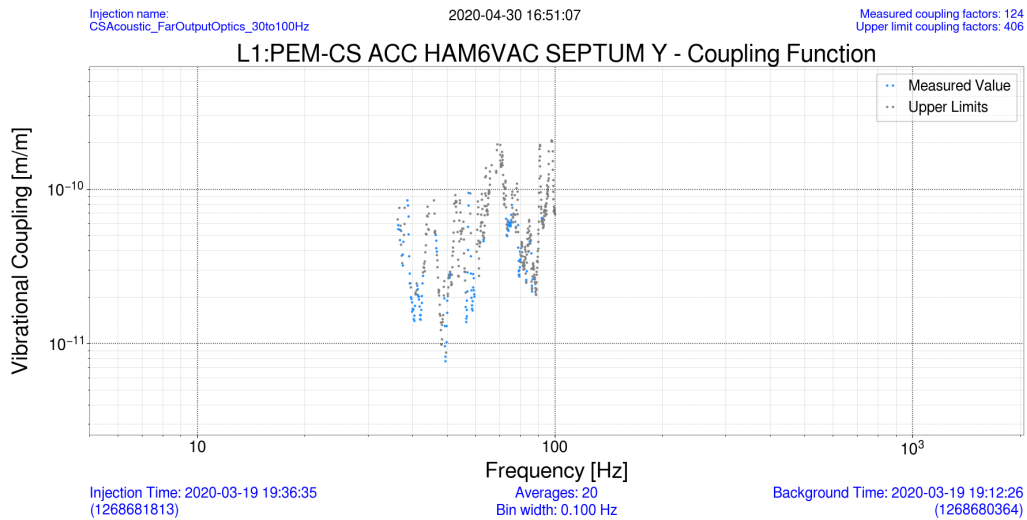
Figure A.2. Coupling function in physical units for the Y-axis HAM 5/6 septum accelerometer from a broadband acoustic injection.
