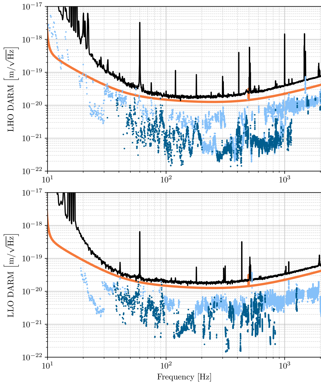
Figure 17. DARM noise from all vibrational coupling sources at LHO (top) and LLO (bottom). Dark blue dots represent measurements, while light blue dots represent upper limits. The black and orange curves show the O3 sensitivity and design sensitivity, respectively.
