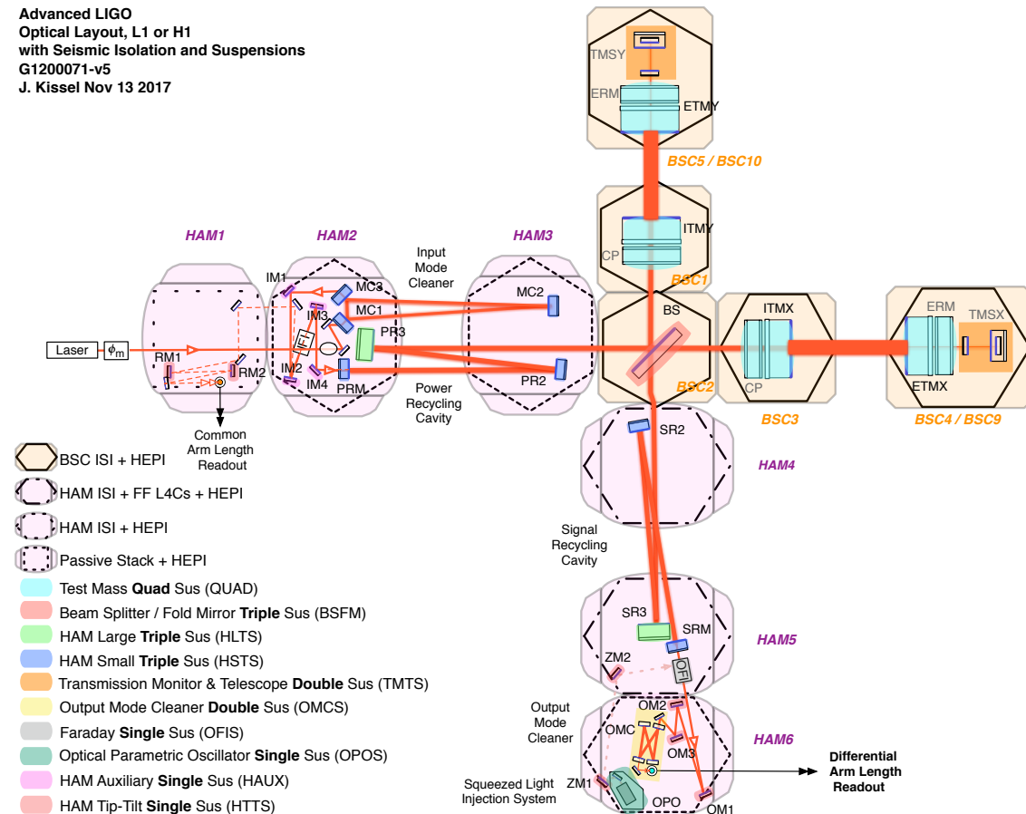
Figure 4. Full optical layout of an Advanced LIGO interferometer (Kissel, 2017).
