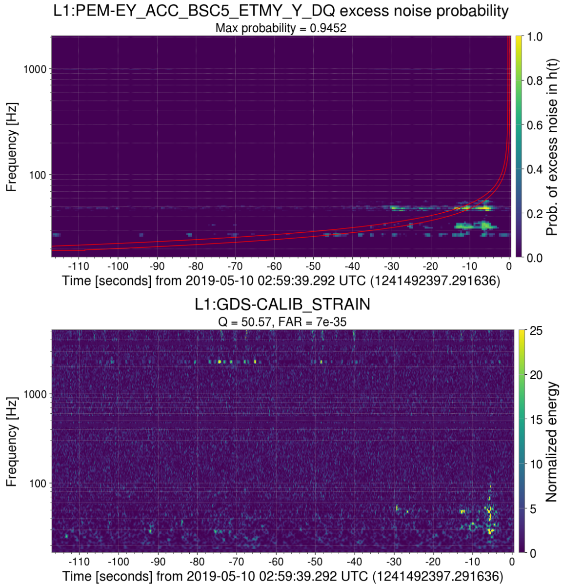
Figure 28. Probability spectrogram of an ETMY accelerometer at LLO (top) and a constant-Q transform of the GW strain channel (bottom). The red lines show the time-frequency path of GW event candidate S190510g.
