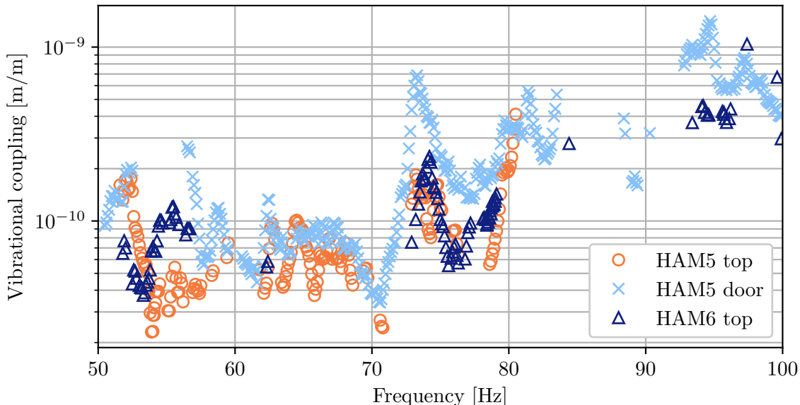
Figure 14. Single-injection coupling functions (upper limits not shown) for the HAM5 Y-axis accelerometer for three different shaker injection locations (on top of HAM5, on top of HAM6, and on the HAM5 chamber door).
