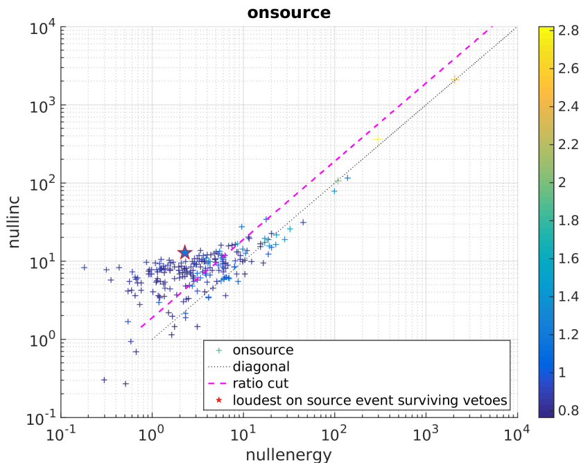
Figure 31. Coherent consistency cut performed by x-pipeline to veto noise triggers. The x - and y -axes represent E_{\text{null}} and I_{\text{null}} , respectively.
