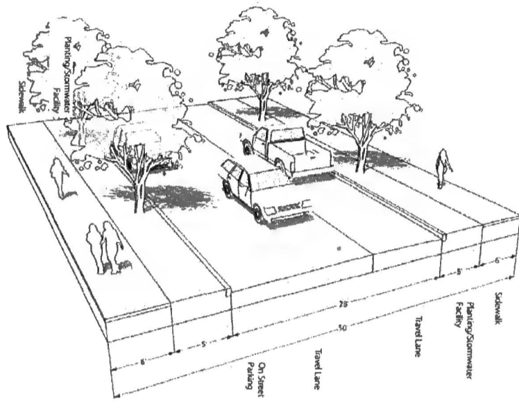
LOCAL STREET I - Two Travel Lanes with On-Street Parking on One side only
