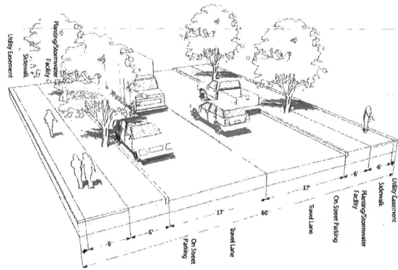
LOCAL STREET II - Two Travel Lanes with On-Street Parking on Both sides
