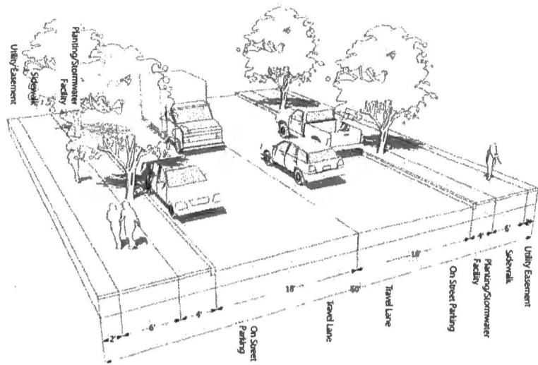
COLLECTOR - Two Travel Lanes with On-Street Parking Both Sides
