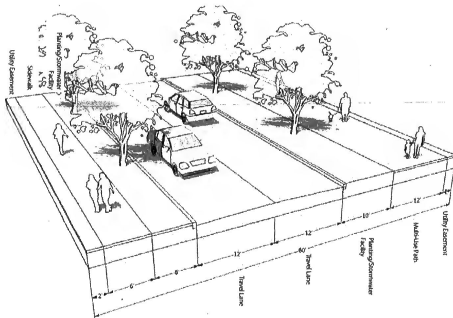
PARKWAY COLLECTOR - Two Travel Lanes with no On-Street Parking
