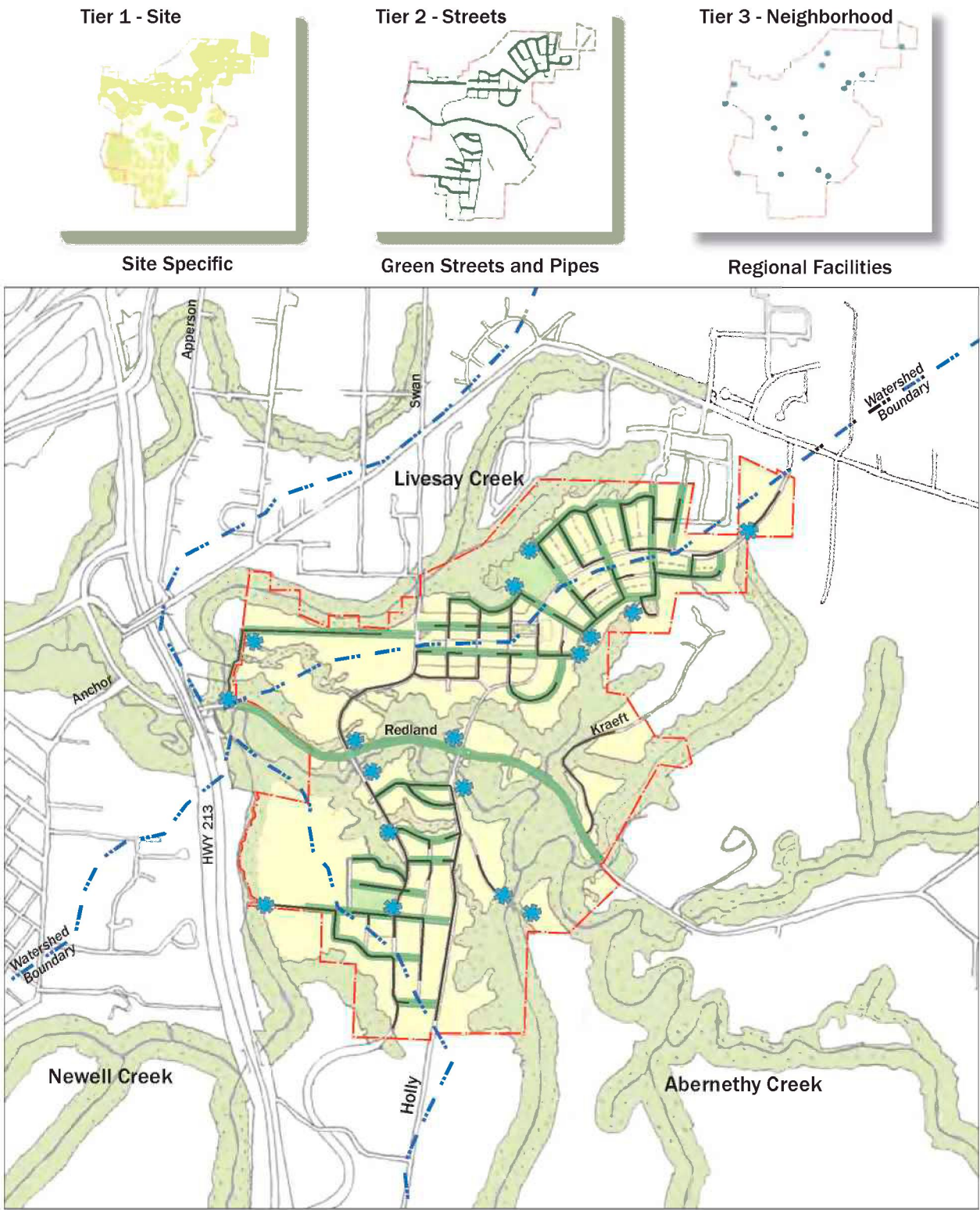
Figure 3-12. Proposed Stormwater Management
