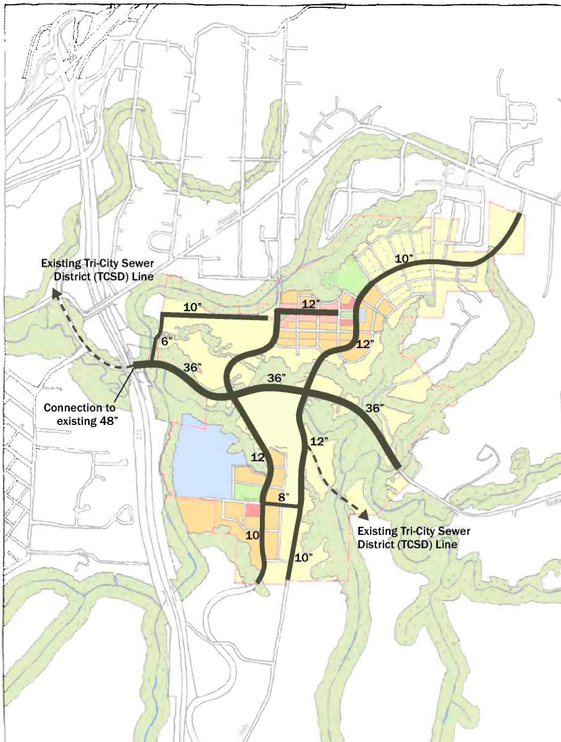
Figure 3-11. Proposed Wastewater System Improvements
