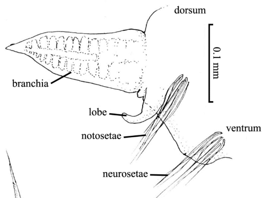
3. Parapodium 13 x250.
