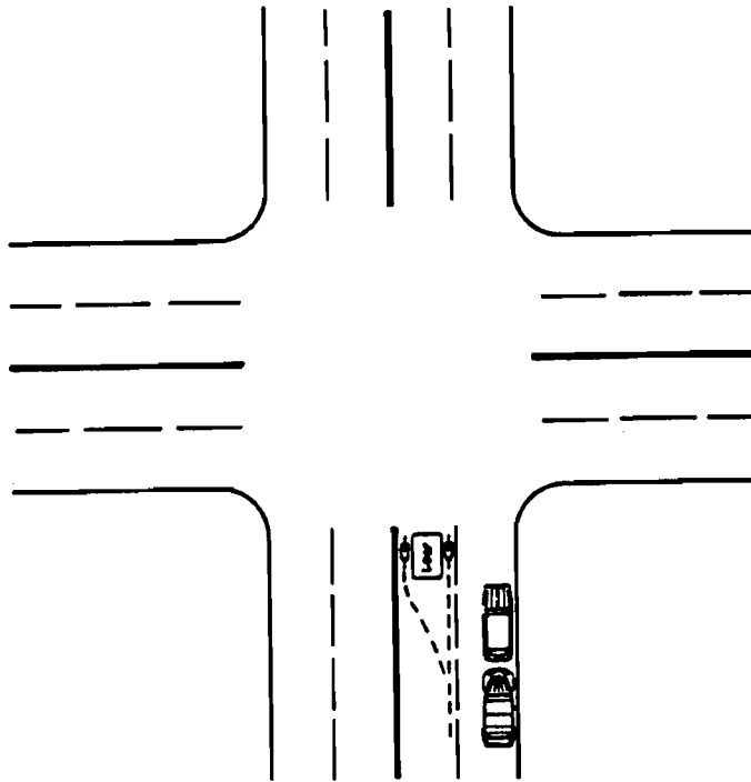
FIGURE 16 - UNDETECTED BICYCLE POSITIONING
